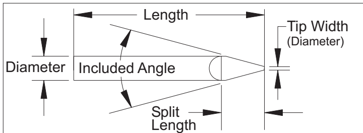
Conical Ballnose Tool
