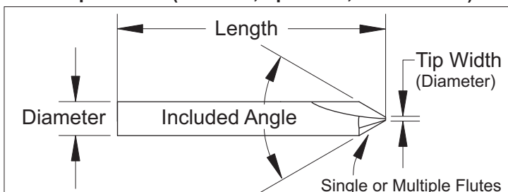
Tough Tip Tool or Engraving Mill-Drill Multiple Flutes (Chamfer, Spot Drill, Countersink)
