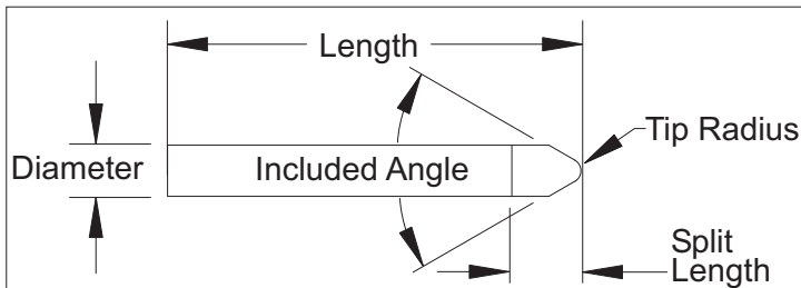
Conical Ballnose Tool
